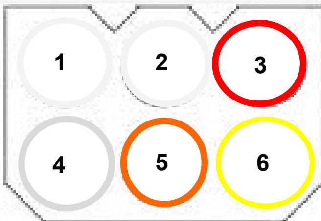
Female Housing
